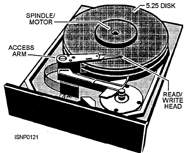
Figure 8-7.—Internal hard-disk drive.
